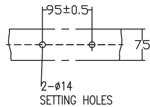
SETTING DIMENSION
