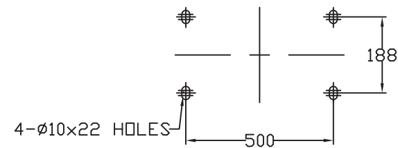
SETTING DIMENSION
